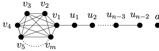
Figure 4. L_{m,n}^{ab} - b .
