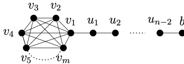
Figure 3. L_{m,n} - a .
