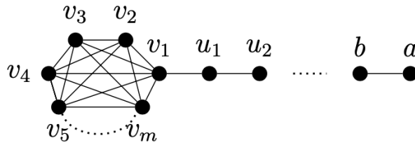
Figure 2. L_{m,n} .
